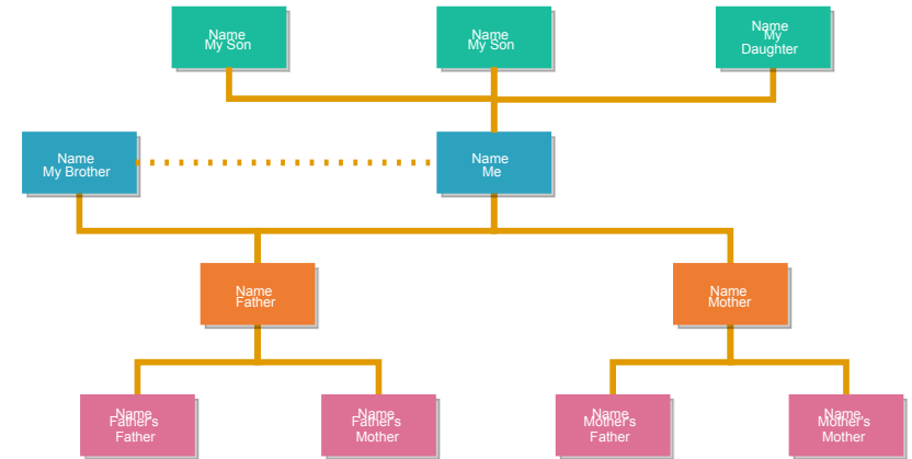
Tree Diagram
