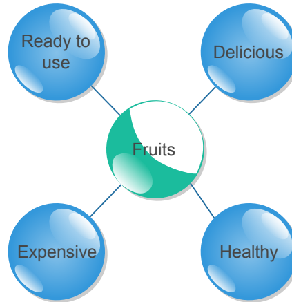
Bubble Diagram
